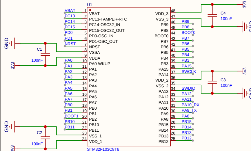
STM32F103CXXX
