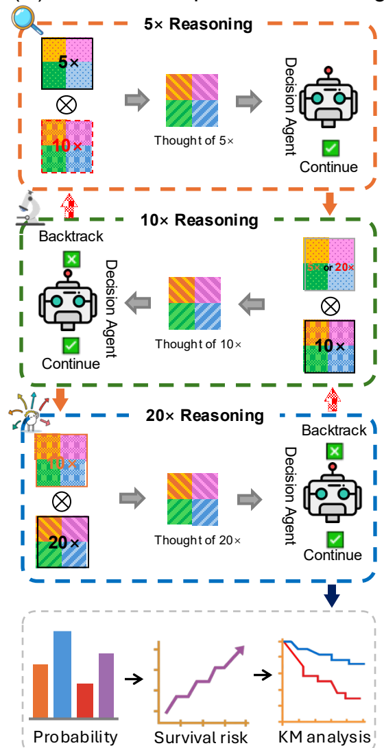
(C) CoT with Adaptive Backtracking
