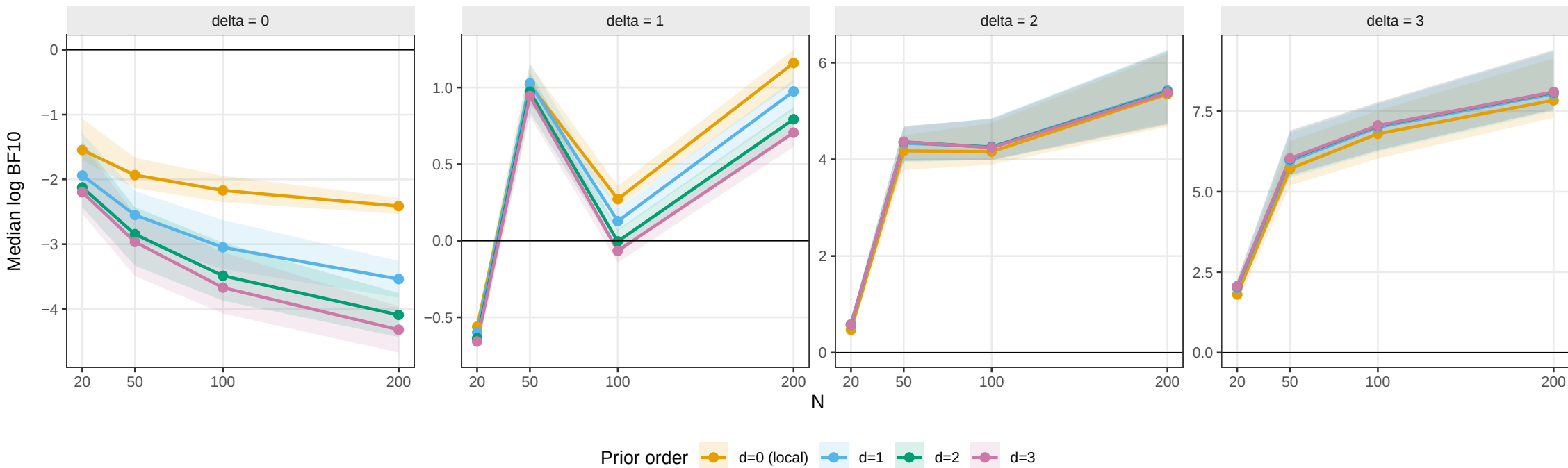
Reweighted interval-null BF from d=0 posterior [logspline, eps = 0.2]
