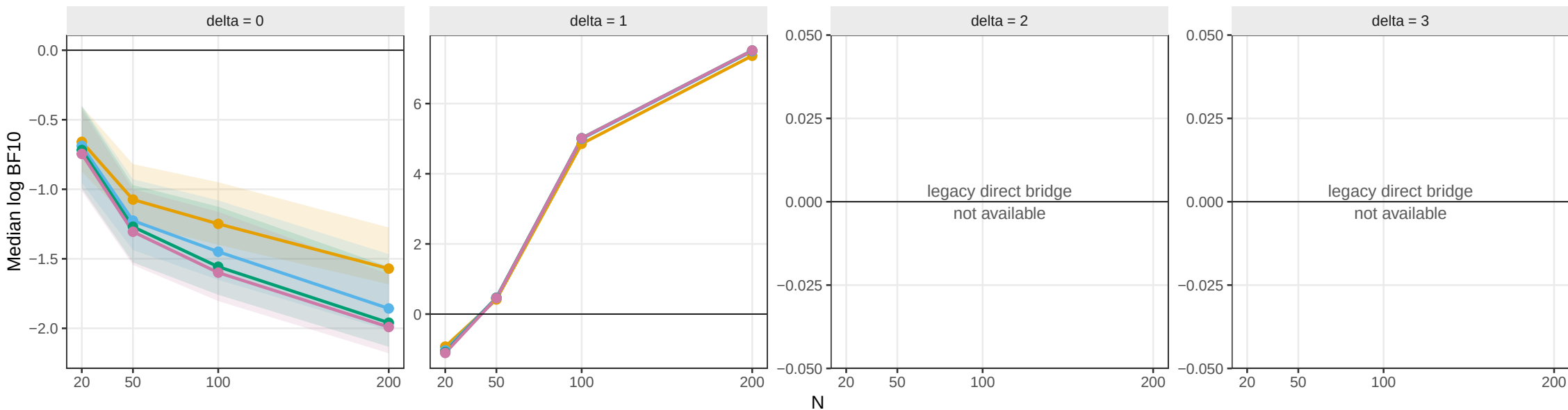
Reweighted interval-null BF from d=0 posterior [logspline, eps = 0.2]
