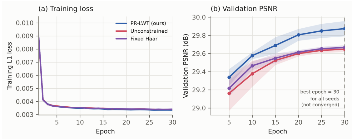
Fig. 14. Convergence dynamics: (a) training L_1 and (b) validation PSNR, three arms, mean \pm 1 SD over five seeds. The two panels use separate x axes — validation runs every fifth epoch, so it has six points against the training curve’s thirty; plotting both on one axis would compress the time axis fivefold. PR-LWT is ahead on both metrics (final-epoch training L_1 0.003346 against 0.003396 and 0.003414). The dashed line in (b) marks that every seed’s best epoch is the last one — i.e. training has not converged, which is limitation 4.
