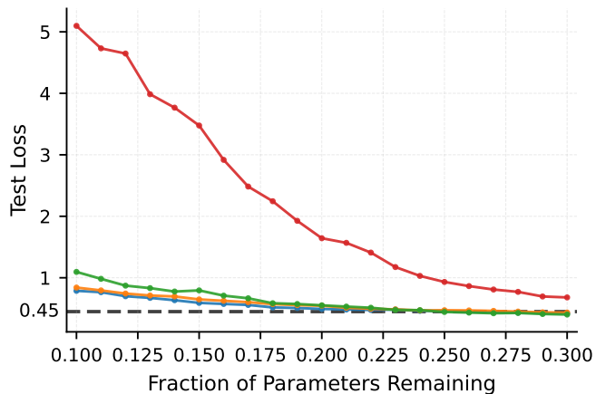
StrongRRQR ARP Baseline RPCholesky Magnitude
