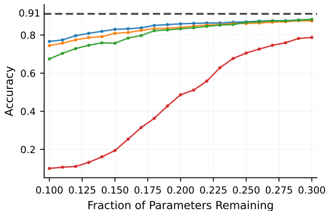
StrongRRQR ARP Baseline RPCholesky Magnitude
