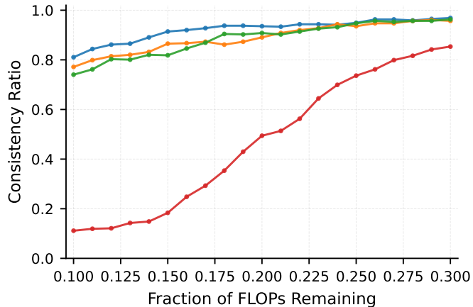
StrongRRQR ARP Magnitude RPCholesky
