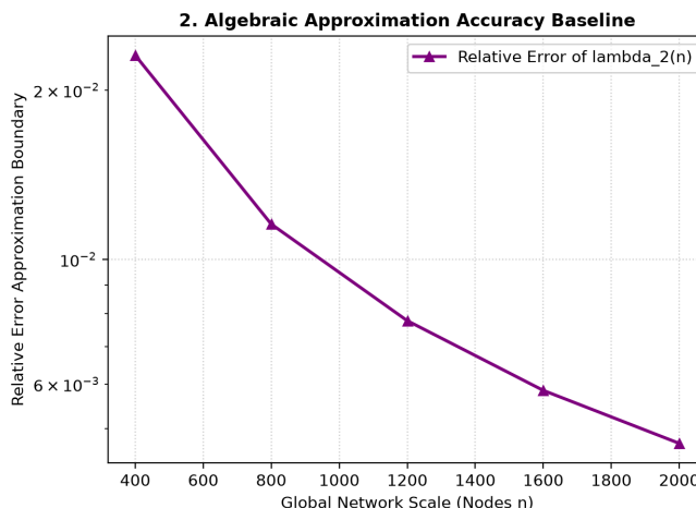
Operator 6 (Psieve U Osplice) Computational Complexity and Accuracy Clamping
