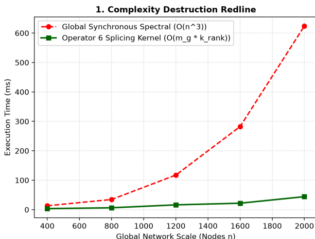
Operator 6 (Psieve U Osplice) Computational Complexity and Accuracy Clamping
