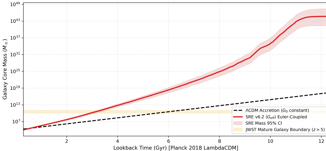
Figure 2: Primordial Mass Accumulation — \Lambda CDM vs SRE v6.2 Ensemble
