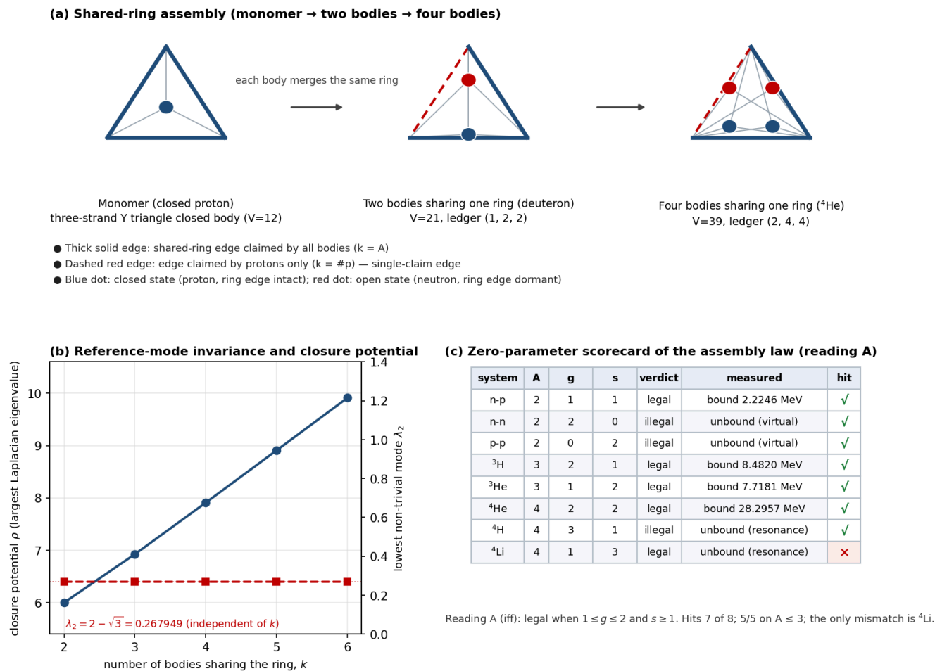
Figure 5: Many-body assembly law and the shared ring. (a) The monomer skeleton is assembled into a k-body shared ring by "merging the same ring (three vertices) into the shared region": thick solid edges are claimed by all bodies ( k=A ), the dashed red edge is a single-claim edge claimed by protons only ( k=\#p ), blue dots are closed states and red dots open states; (b) the closure potential \rho rises monotonically with the body count, whereas the lowest non-trivial mode \lambda_2 = 2-\sqrt{3} is independent of the body count (reference mode; the data are independently recomputed by the companion script from numerical Laplacian spectra, with a
