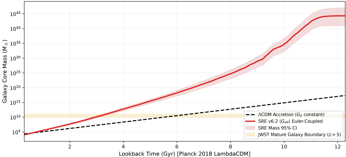
Figure 2: Primordial Mass Accumulation — \Lambda CDM vs SRE v6.2 Ensemble
