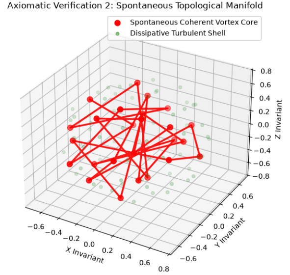
Figure 1. Axiomatic numerical verification of the SRE-MDS discrete pipeline under zero-boundary constraints.
