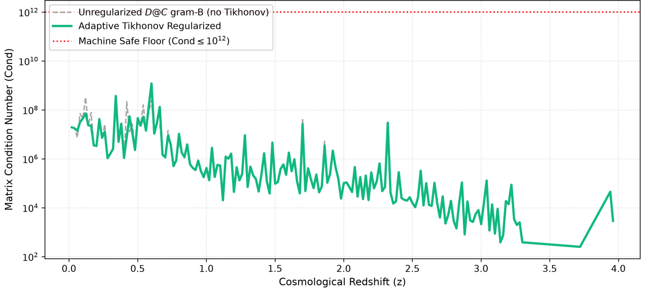
Figure 3: Numerical Stability Monitor — D@C Matrix Product
