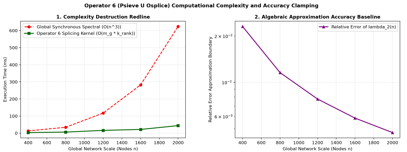
Figure-1: Numerical verification suite for Operator 6.
