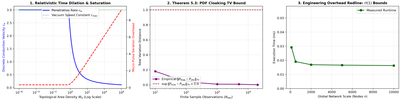
Figure-1: Numerical verification suite for Operator 5.
