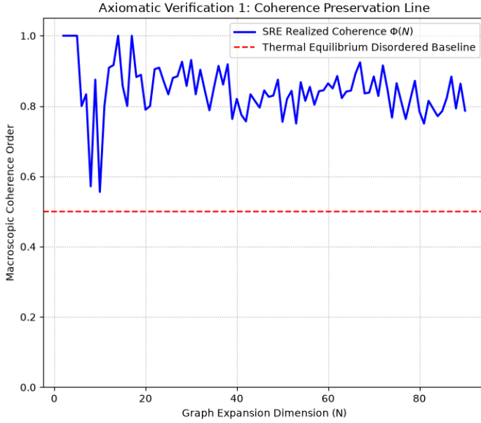
Figure 1. Axiomatic numerical verification of the SRE-MDS discrete pipeline under zero-boundary constraints.
