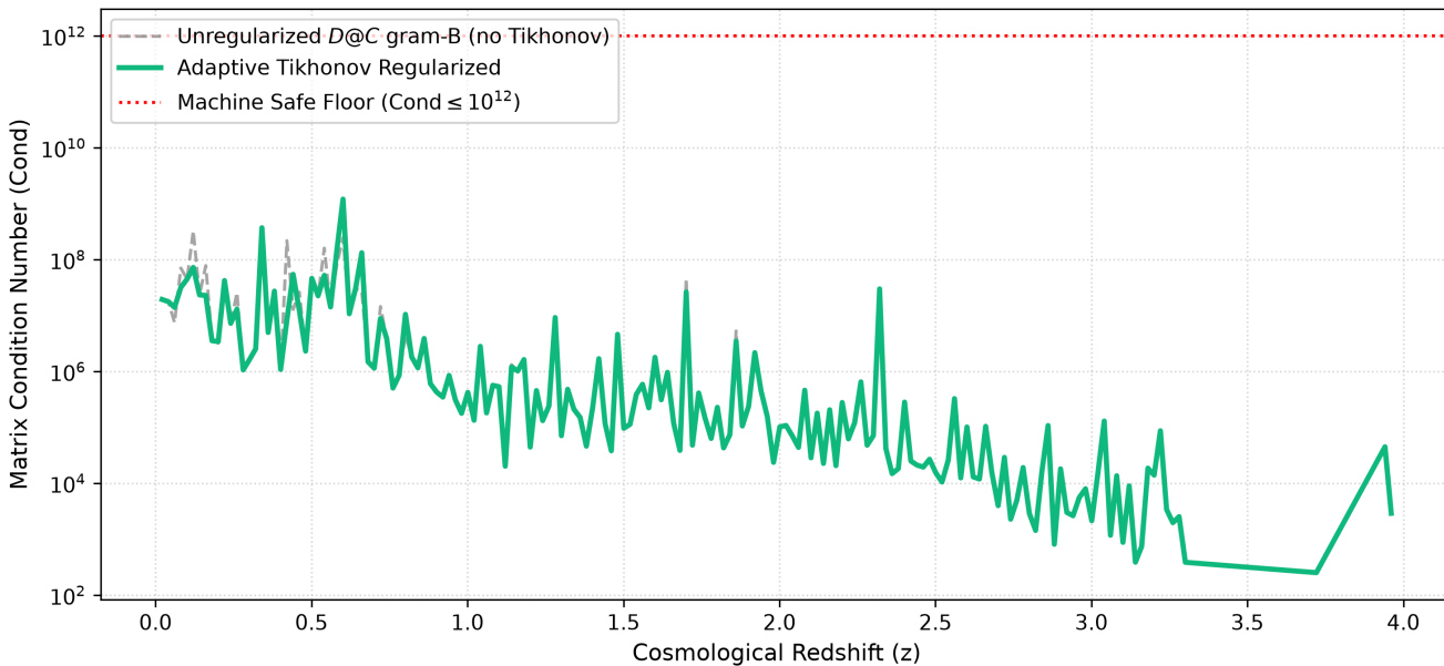
Figure 3: Numerical Stability Monitor — D@C Matrix Product
