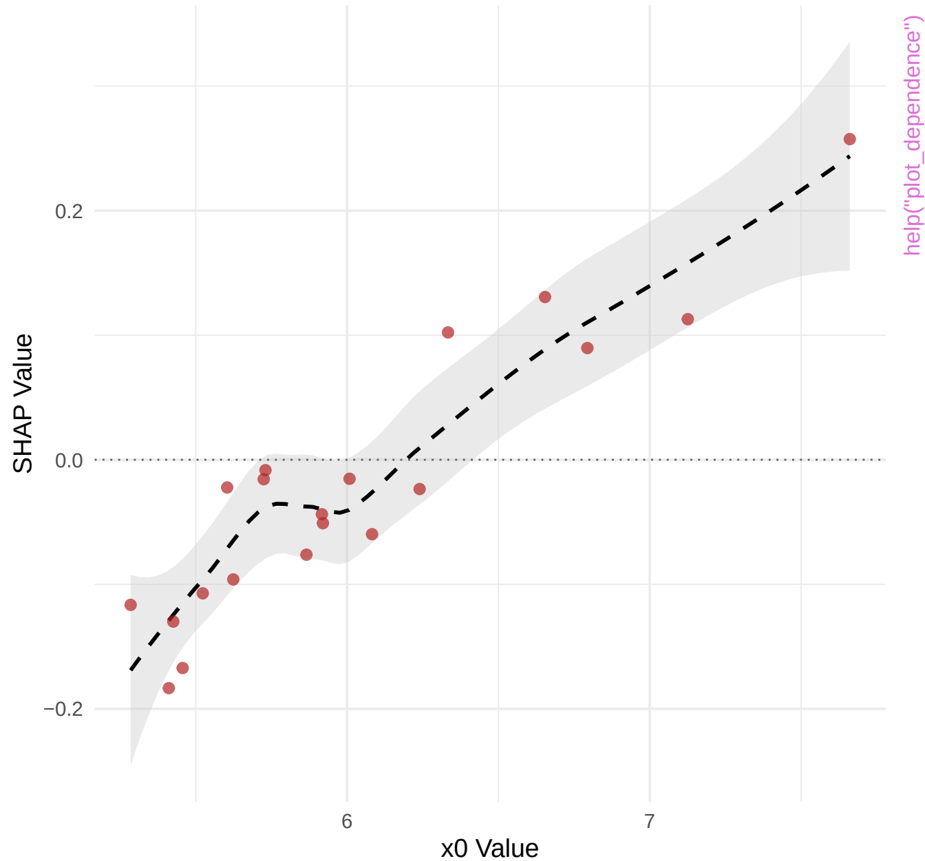
SHAP Dependence: x0
