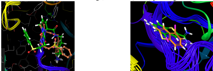
(a) Thrombin: rotational misorientation. The ligand’s bulky substituent is rotated toward the wrong catalytic-pocket residue.
