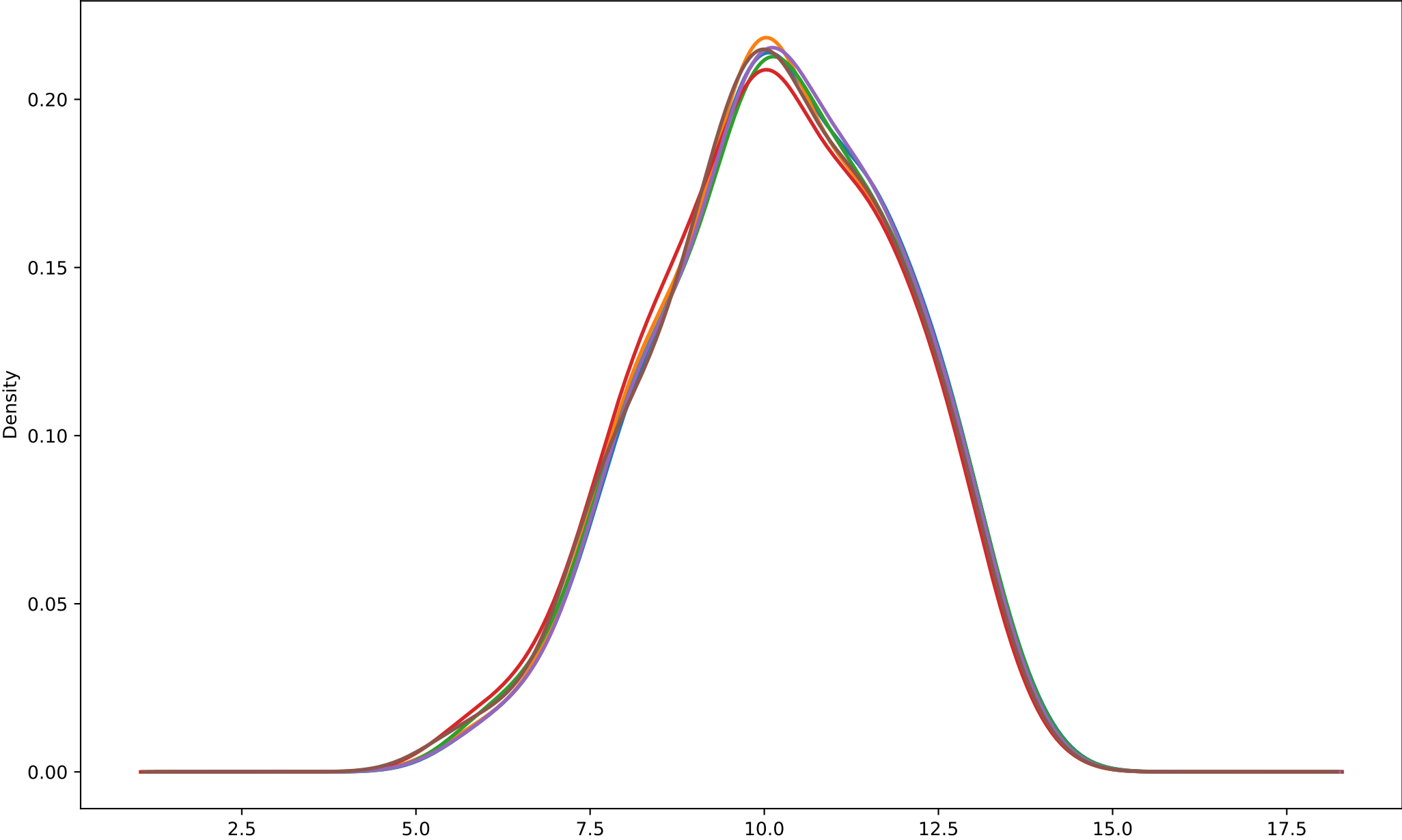
Concentration[nM] Distribution
