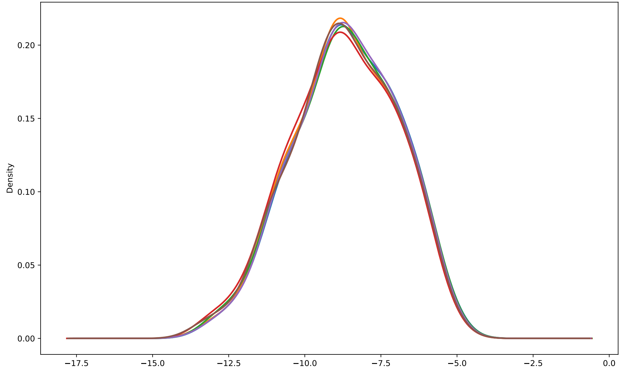
TPA Distribution
