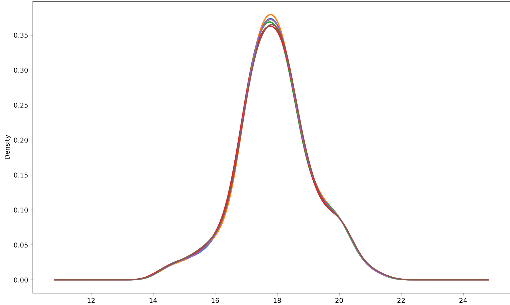
IbaqPpb Distribution
