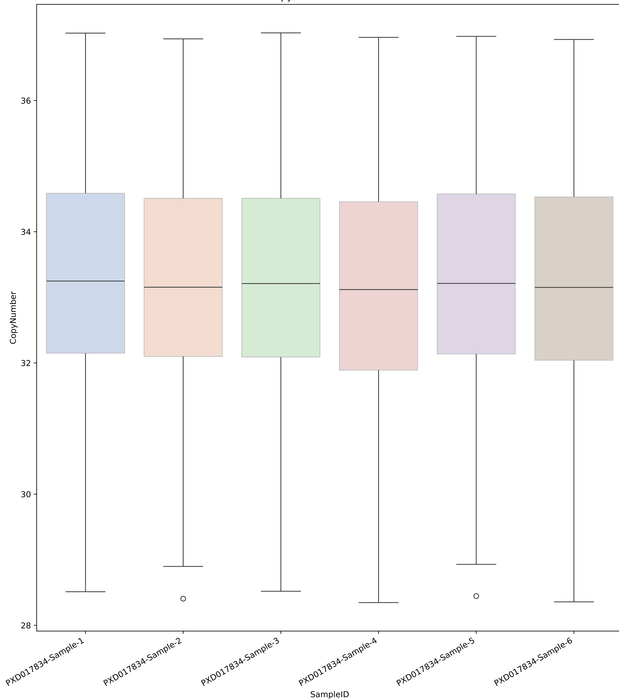
CopyNumber Distribution
