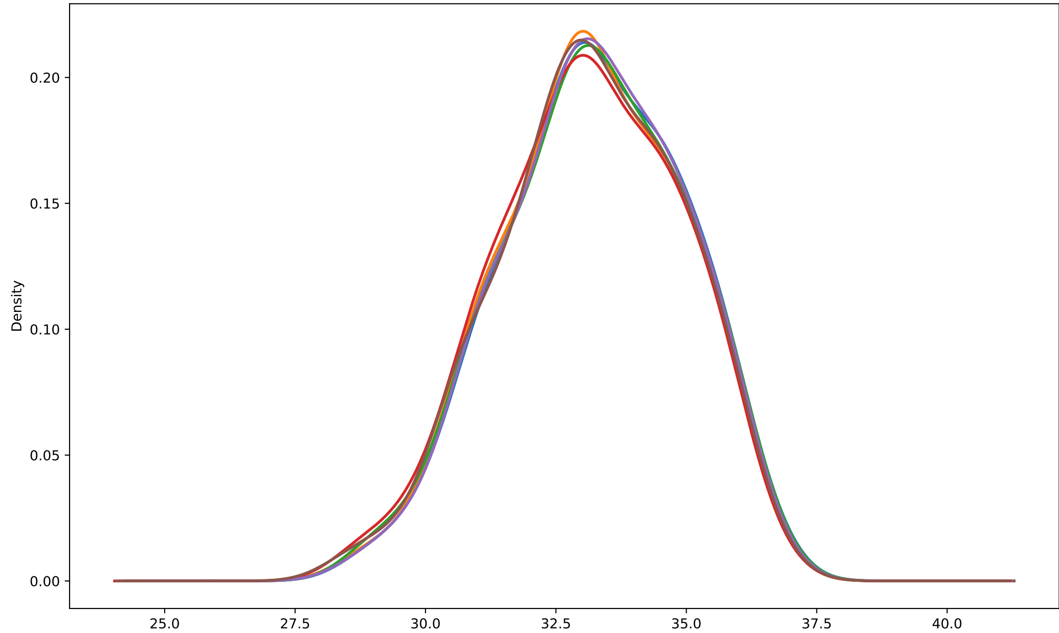
CopyNumber Distribution
