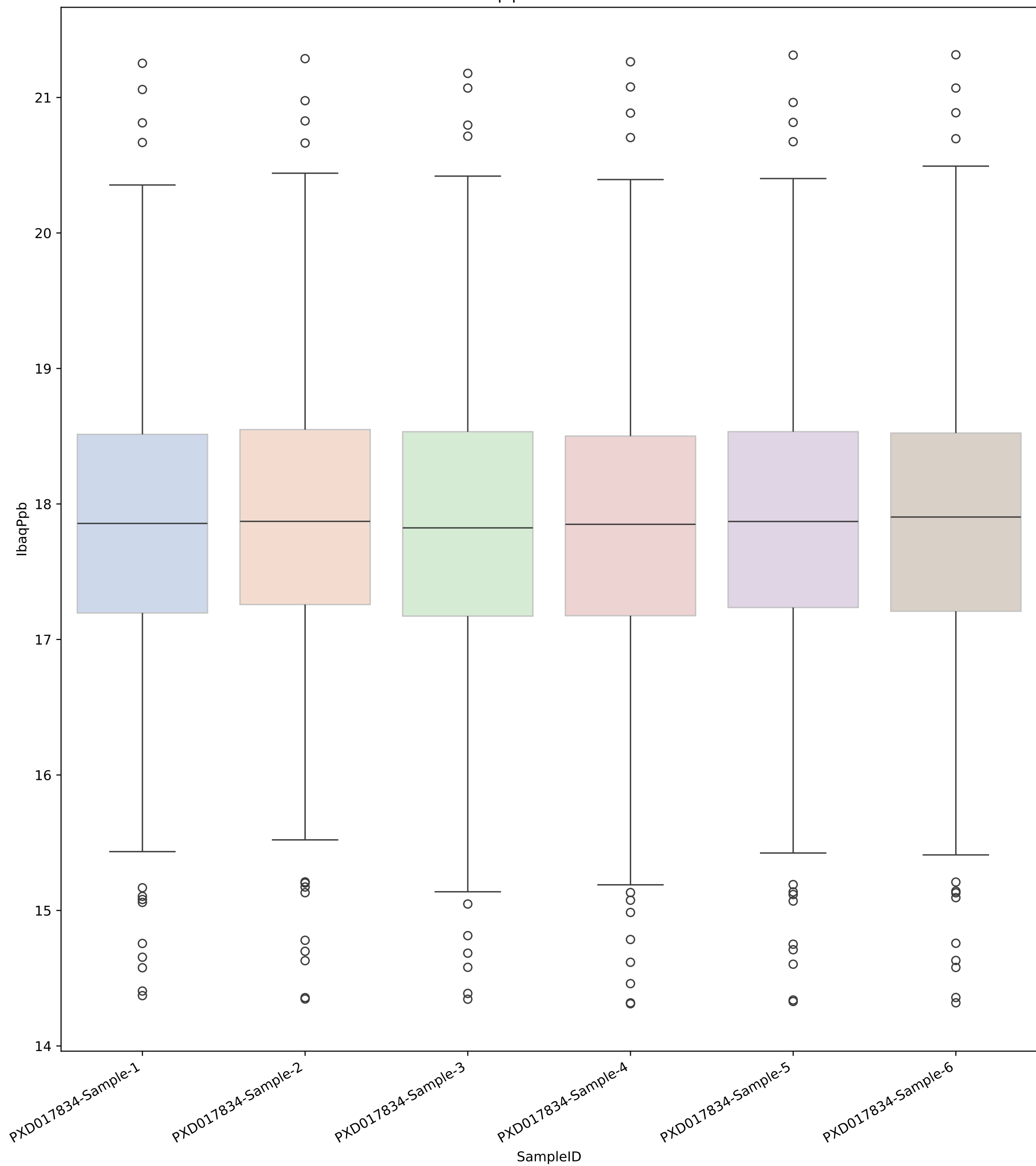
IbaqPpb Distribution
