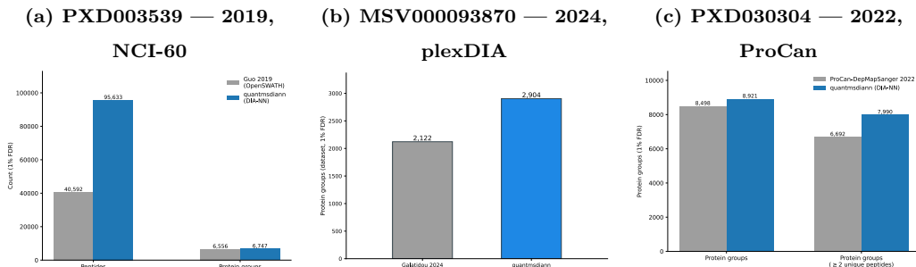
Figure 3: Independent reanalysis of public DIA datasets recovers as many or more identifications than the original deposits. Each panel compares the original published counts (grey) with the quantmsdiann reanalysis at 1% FDR (blue) from the same raw data. (a) NCI-60 bulk cell lines (PXD003539, Guo 2019; original OpenSWATH analysis). (b) Single-cell oocyte plexDIA (MSV000093870, Galatidou 2024). (c) ProCan-DepMapSanger pan-cancer cell-line panel (PXD030304). Per-cohort detail in Additional file 1: Figs. S5–S13.
