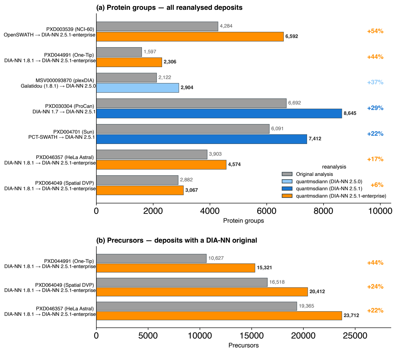
Figure 4: Reanalysis with current DIA-NN recovers more than the originally deposited analyses. Each public DIA deposit is shown as the originally deposited or published count (grey) versus the quantmsdiann reanalysis (coloured by the DIA-NN version used: 2.5.0, 2.5.1, or 2.5.1-enterprise), sorted by gain. (a) Protein groups for all seven reanalysed deposits, spanning single-cell (HeLa Astral, PXD046357; One-Tip, PXD044991; plexDIA, MSV000093870), bulk cell-line (NCI-60, PXD003539; ProCan, PXD030304; Sun, PXD004701) and spatial Deep Visual Proteomics (PXD064049). (b) Precursors, restricted to the three deposits with a DIA-NN-based original precursor count (One-Tip, HeLa Astral and spatial DVP); the OpenSWATH/PCT-SWATH originals, and plexDIA (protein-level report only), provide no comparable precursor count. The quantmsdiann side is counted from the precursor report (parquet) and the original side from the deposit's matrix or published headline, each under the like-for-like per-cohort filter (Supplementary Note 3). The five-cohort pan-cohort integration (per-tissue coverage) is in Supplementary Fig. S13.
