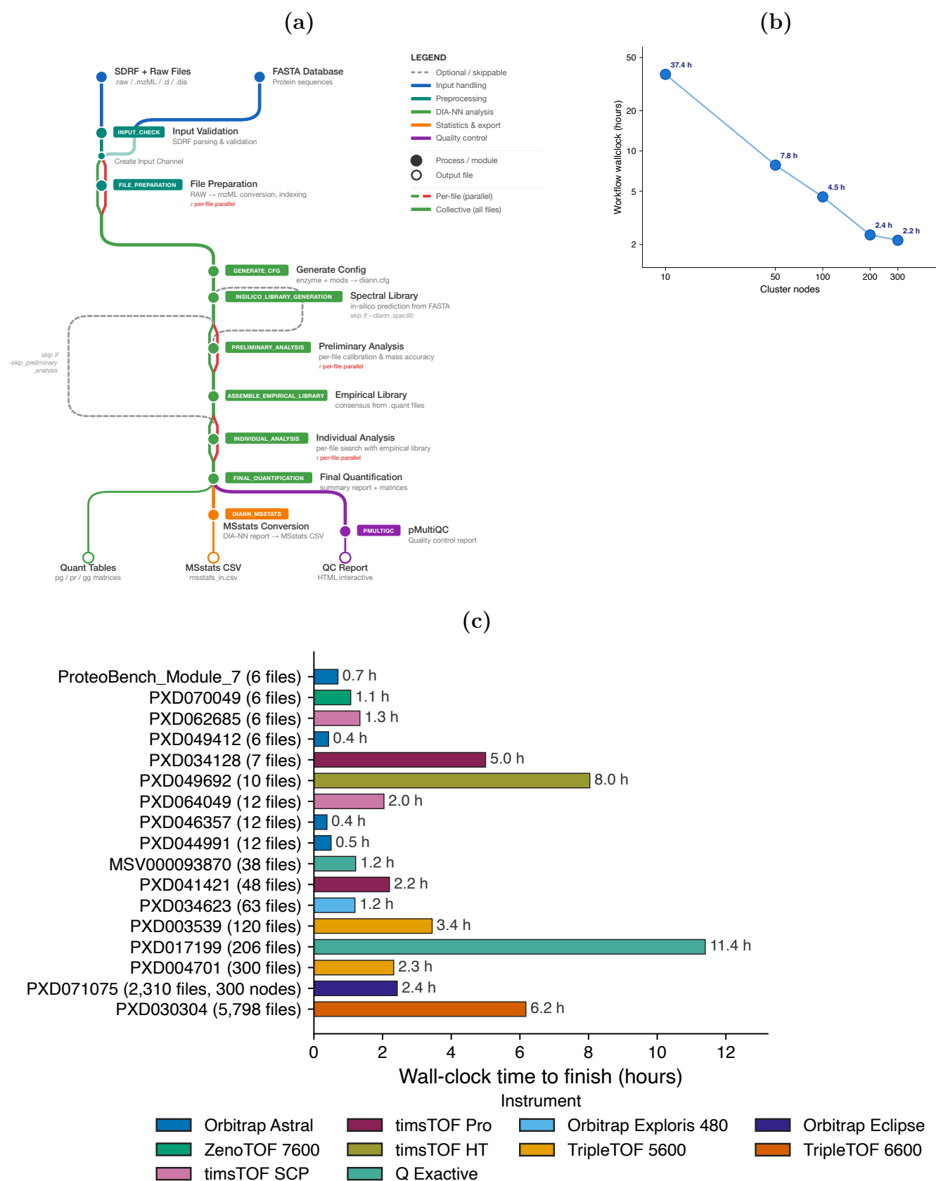
Figure 1: quantmsdiann pipeline architecture and runtime scaling. (a) Subway diagram of the quantmsdiann workflow: mandatory modules as filled circles, optional/skippable modules as open circles. Per-file parallel stages (red; file preparation, preliminary calibration, individual search) run as one task per raw file, whereas collective stages (green; in-silico library generation, empirical library assembly, final quantification, MSstats conversion, and pmultiqc reporting) run once over the full cohort. (b) Workflow wall-clock time versus the number of cluster nodes (Nextflow executor.queueSize ) on the PXD071075 single-cell cohort. (c) Wall-clock time to finish each reanalysis, one bar per dataset, ordered by cohort size (number of MS data files) and coloured by instrument family. In both (b) and (c), the color of the bars corresponds to the instrument family used for data acquisition (Orbitrap Astral, ZenoTOF 7600, timsTOF SCP, timsTOF Pro, timsTOF HT, Q Exactive, Orbitrap Exploris 480, TripleTOF 5600, Orbitrap Eclipse, TripleTOF 6600).
