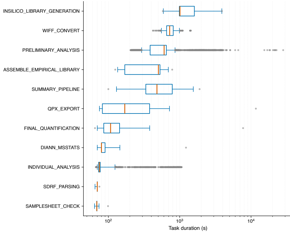
Figure S1: Per-step wall-clock distribution across Nextflow processes. Distribution of task wall-clock time (boxplot, median and IQR) for each quantmsdiann process across the ProteoBench benchmark cohorts and the PXD071075 cluster-node sweep. The per-file parallel stages ( FILE_PREPARATION , PRELIMINARY_ANALYSIS , INDIVIDUAL_ANALYSIS ) run as one task per raw file and determine the workflow's parallelisation envelope, while the collective stages ( INSILICO_LIBRARY_GENERATION , ASSEMBLE_EMPIRICAL_LIBRARY , FINAL_QUANTIFICATION , DIANN_MSSTATS ) run once per cohort and set the wall-clock floor at maximum cluster width.
