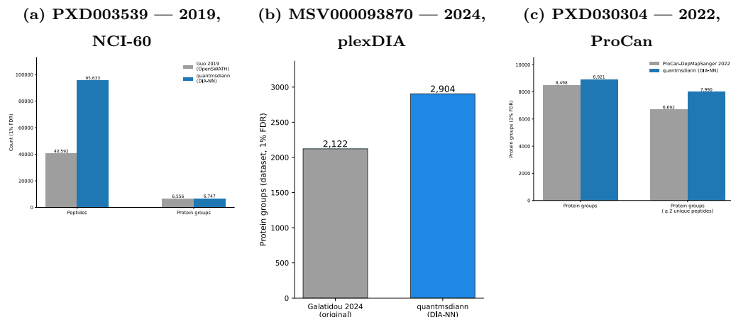
Figure 3: Independent reanalysis of public DIA datasets, spanning bulk cell lines and single cells, recovers as many or more identifications than the originally deposited quantifications. Each panel compares the originally published peptide and/or protein-group counts (grey) against the quantmsdiann reanalysis at 1% FDR (blue) using the same raw data. (a) Guo et al. , 2019 NCI-60 OpenSWATH analysis (PXD003539, original engine = OpenSWATH with the Guo 2019 assay library): quantmsdiann recovers 95,633 peptides versus 40,592 originally (+135%) and a comparable 6,747 protein groups versus 6,556. Because quantmsdiann runs DIA-NN in library-free mode while the original ran OpenSWATH against a fixed assay library, this gain reflects both SDRF-driven orchestration and the change of analysis engine; a like-for-like DIA-NN-on-original-library control is part of ongoing work. (b) Galatidou et al. , 2024 single-cell oocyte plexDIA (MSV000093870; mTRAQ 3-channel, Q Exactive): from the same raw data quantmsdiann quantifies 2,904 protein groups versus 2,122 in the original analysis (+37%), recovering 95% of the original accessions plus 1,539 additional proteins at comparable per-cell median depth (1,736 versus 1,784 protein groups; full per-cell, total and accession-overlap comparison in Additional file 1). (c) ProCan-DepMapSanger 2022 pan-cancer cell-line panel (PXD030304, 949 lines): quantmsdiann recovers 8,921 protein groups at 1% FDR versus 8,498 originally (+5%), and 7,990 versus 6,692 after requiring \geq 2 unique peptides per protein (+19%). Both the original 8,498 headline (Global.Q.Value \leq 0.01 ) and the stringent 6,692 count (Global.Q.Value \leq 0.01 plus \geq 2 supporting peptides) are reported in the ProCan-DepMapSanger paper itself; the quantmsdiann counts are computed under the matching filters, so each side of the comparison is like-for-like. Per-condition completeness, peptide-per-protein distributions and gene- versus accession-level overlap are shown in Additional file 1: Figs. S5–S13.
