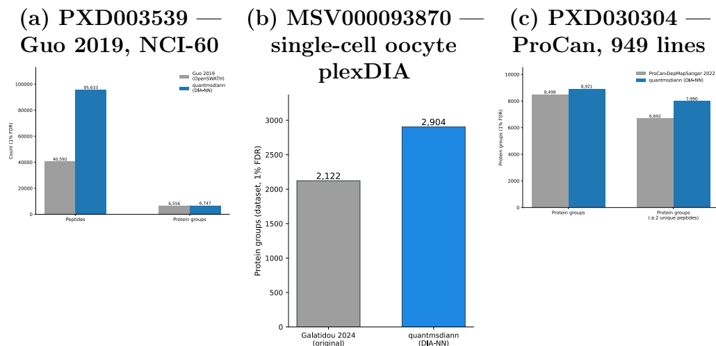
Figure 3: Independent reanalysis of public DIA datasets, spanning bulk cell lines and single cells, recovers as many or more identifications than the originally deposited quantifications. Each panel compares the originally published peptide and/or protein-group counts (grey) against the quantmsdiann reanalysis at 1% FDR (blue) using the same raw data. (a) Guo et al. , 2019 NCI-60 OpenSWATH analysis (PXD003539, original engine = OpenSWATH with the Guo 2019 assay library): quantmsdiann recovers 95,633 peptides versus 40,592 originally (+135%) and a comparable 6,747 protein groups versus 6,556. Because quantmsdiann runs DIA-NN in library-free mode while the original ran OpenSWATH against a fixed assay library, this gain reflects both SDRF-driven orchestration and the change of analysis engine; a like-for-like DIA-NN-on-original-library control is part of ongoing work. (b) Galatidou et al. , 2024 single-cell oocyte plexDIA (MSV000093870; mTRAQ 3-channel, Q Exactive): from the same raw data quantmsdiann quantifies 2,904 protein groups versus 2,122 in the original analysis (+37%), recovering 95% of the original accessions plus 1,539 additional proteins at comparable per-cell median depth (1,736 versus 1,784 protein groups; full per-cell, total and accession-overlap comparison in Additional file 1). This is the first plexDIA cohort processed through quantmsdiann . (c) ProCan-DepMapSanger 2022 pan-cancer cell-line panel (PXD030304, 949 lines): quantmsdiann recovers 8,921 protein groups at 1% FDR versus 8,498 originally (+5%), and 7,990 versus 6,692 after requiring \geq 2 unique peptides per protein (+19%). Both the original 8,498 headline (Global.Q.Value \leq 0.01 ) and the stringent 6,692 count (Global.Q.Value \leq 0.01 plus \geq 2 supporting peptides) are reported in the ProCan-DepMapSanger paper itself; the quantmsdiann counts are computed under the matching filters, so each side of the comparison is like-for-like. Per-condition completeness, peptide-per-protein distributions and gene- versus accession-level overlap are shown in Additional file 1: Figs. S5–S10.
