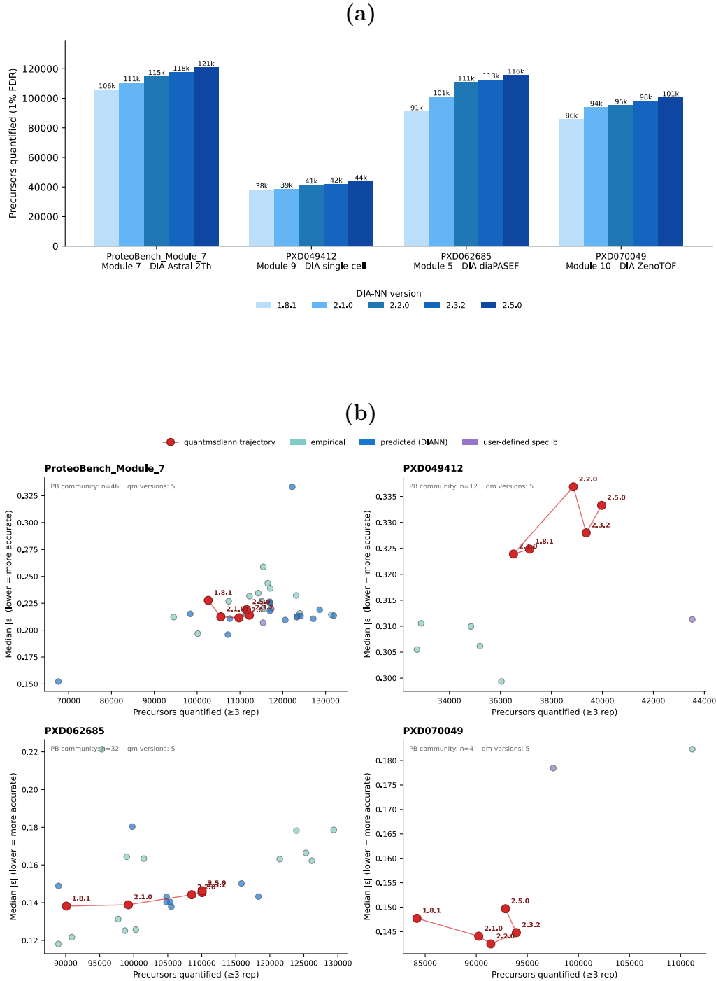
Figure 2: quantmsdiann on ProteoBench across five DIA-NN releases and four DIA modalities. Four ProteoBench DIA modules cover Orbitrap Astral (Module 7), single-cell DIA (Module 9, PXD049412), timsTOF diaPASEF (Module 5, PXD062685) and SCIEX ZenoTOF (Module 10, PXD070049). (a) Precursors at 1% FDR by DIA-NN version (1.8.1–2.5.0; light to dark blue) from one quantmsdiann invocation; identification counts grow monotonically with version (e.g. Module 5 91,075 → 115,735). (b) Precursors quantified ( \geq 3 replicates) versus median |\epsilon| for every public ProteoBench submission per module (snapshot [snapshot date YYYY-MM-DD]; coloured by library mode); the quantmsdiann trajectory across the five DIA-NN versions is overlaid in red. Note that, unlike the identification-count trend in panel (a), median |\epsilon| does not always decrease with the newest DIA-NN version: per module the best identification–accuracy trade-off may sit at an intermediate version. Users
