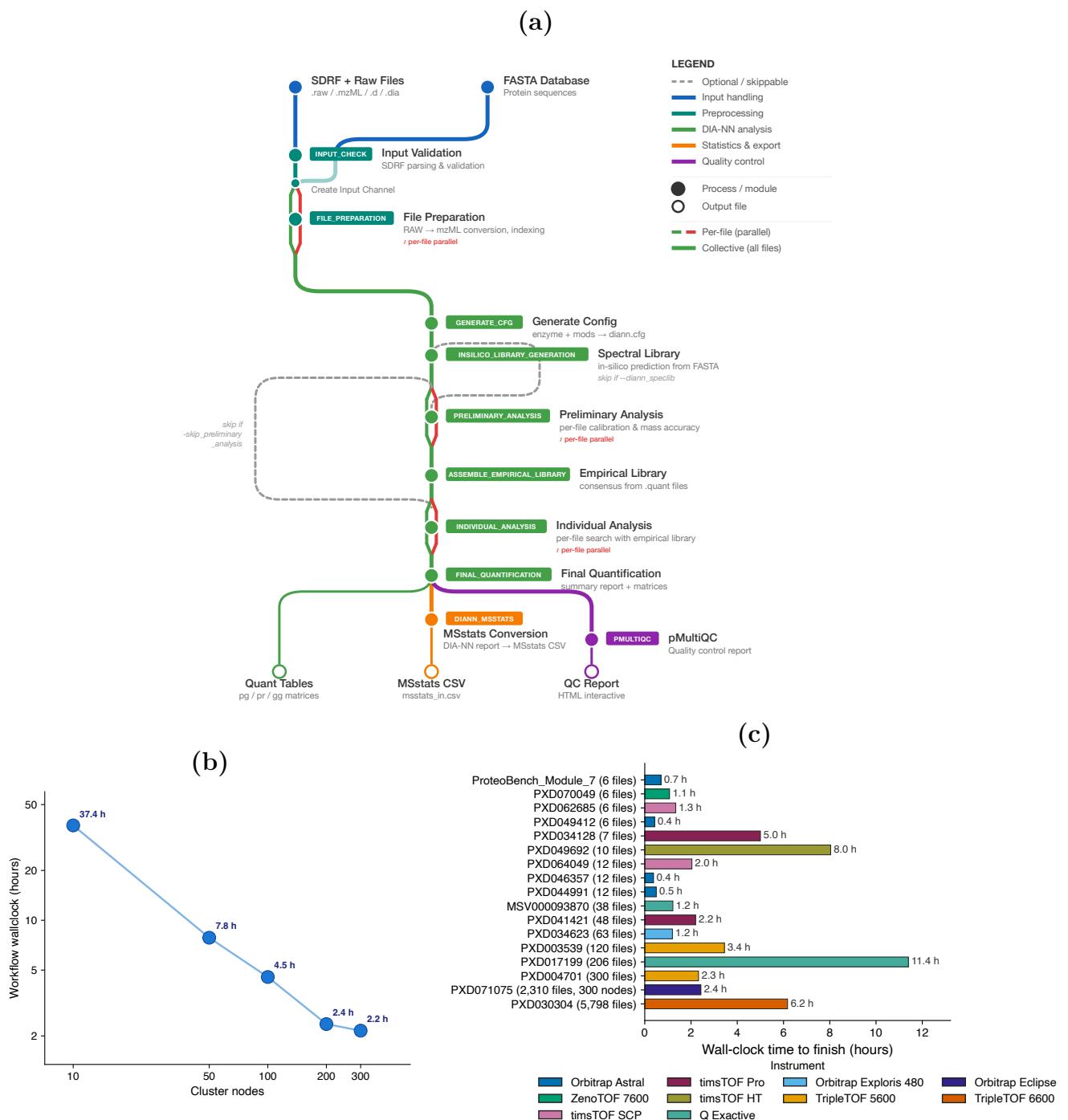
Figure 1: quantmsdiann pipeline architecture and runtime scaling. (a) Subway diagram of the quantmsdiann workflow: mandatory modules as filled circles, optional/skippable modules as open circles. Per-file parallel stages (red; file preparation, preliminary calibration, individual search) run as one task per raw file, whereas collective stages (green; in-silico library generation, empirical library assembly, final quantification, MSstats conversion, and pmultiqc reporting) run once over the full cohort. (b) Workflow wall-clock time versus the number of cluster nodes (Nextflow executor.queueSize ) on the PXD071075 single-cell cohort. (c) Wall-clock time to finish each reanalysis, one bar per dataset, ordered by cohort size (number of MS data files) and coloured by instrument family. In both (b) and (c) the reported time excludes the in-silico spectral-library prediction step ( INSILICO_LIBRARY_GENERATION ), a one-time, cohort-independent cost that can be predicted once and reused, so the bars reflect the per-file quantification work. Time-to-finish stays within a few hours across two orders of magnitude in file count because per-file stages are parallelised across the cluster; the deeper variable-modification search of the phosphoproteomics cohorts (e.g. PXD049692) is the main residual driver of wall-clock once library prediction is set aside.
