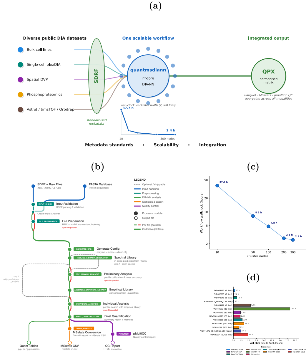
Figure 1: quantmsdiann: SDRF-driven workflow, architecture, and runtime scaling. (a) Conceptual overview: diverse public DIA datasets (bulk, single-cell plexDIA, spatial, phosphoproteomics), each described by one standardised SDRF, are reanalysed by a single nf-core/DIA-NN workflow parallelised across HPC/cloud and exported to one harmonised, queryable QPX archive. (b) Subway diagram of the quantmsdiann workflow: mandatory modules as filled circles, optional/skippable modules as open circles. Per-file parallel stages (red; file preparation, preliminary calibration, individual search) run as one task per raw file, whereas collective stages (green; in-silico library generation, empirical library assembly, final quantification, MSstats conversion, and pmultiqc reporting) run once over the full cohort. (c) Workflow wall-clock time versus the number of cluster nodes (Nextflow executor.queueSize ) on the PXD071075 single-cell cohort. (d) Wall-clock time to finish each reanalysis, one bar per dataset, ordered by cohort size (number of MS data files) and coloured by instrument family. For proteome-scale cohorts, time-to-finish stays within a few hours regardless of file count because per-file work is parallelised; the longest run is a phosphoproteomics cohort (PXD049692), where generating the deep variable-modification spectral library dominates the wall-clock.
