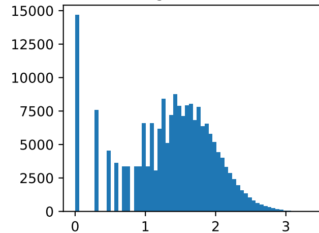
log10 counts
