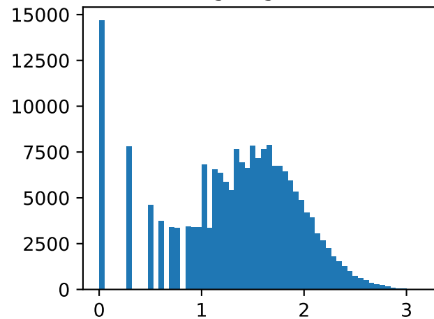
log10 genes
