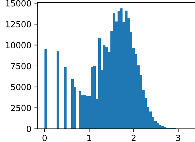
log10 genes
