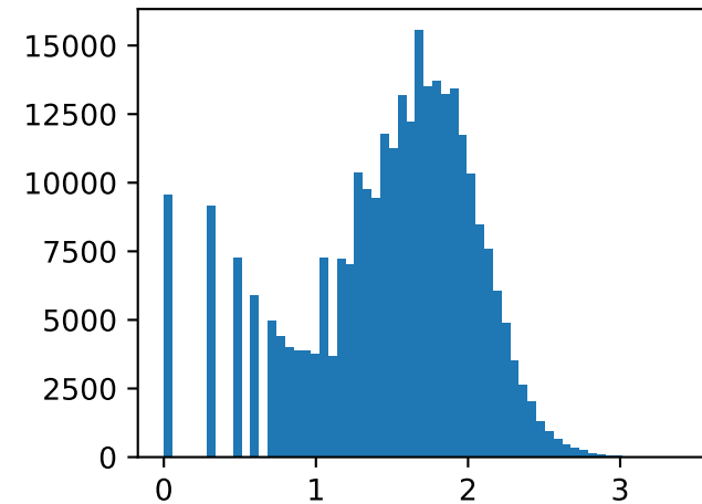
log10 counts
