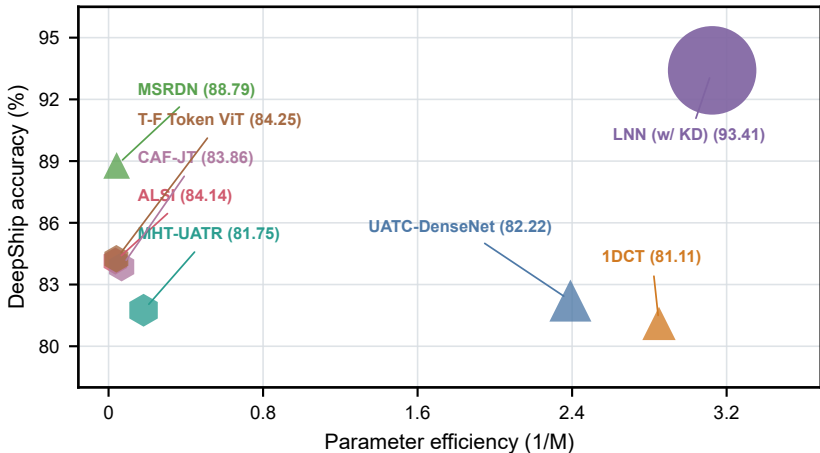
Parameter efficiency vs accuracy
