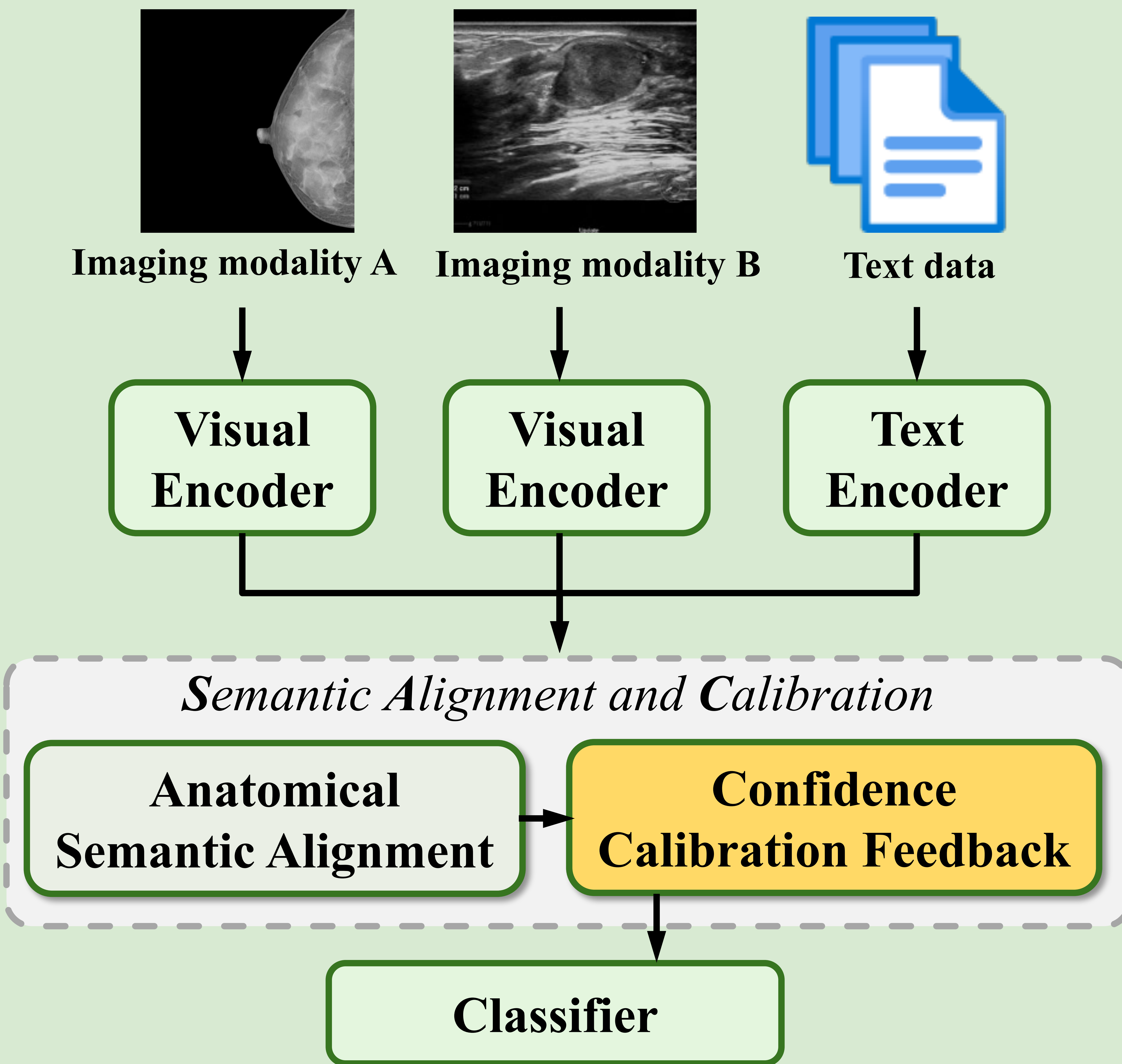
(c) MSAC-Net(ours)
