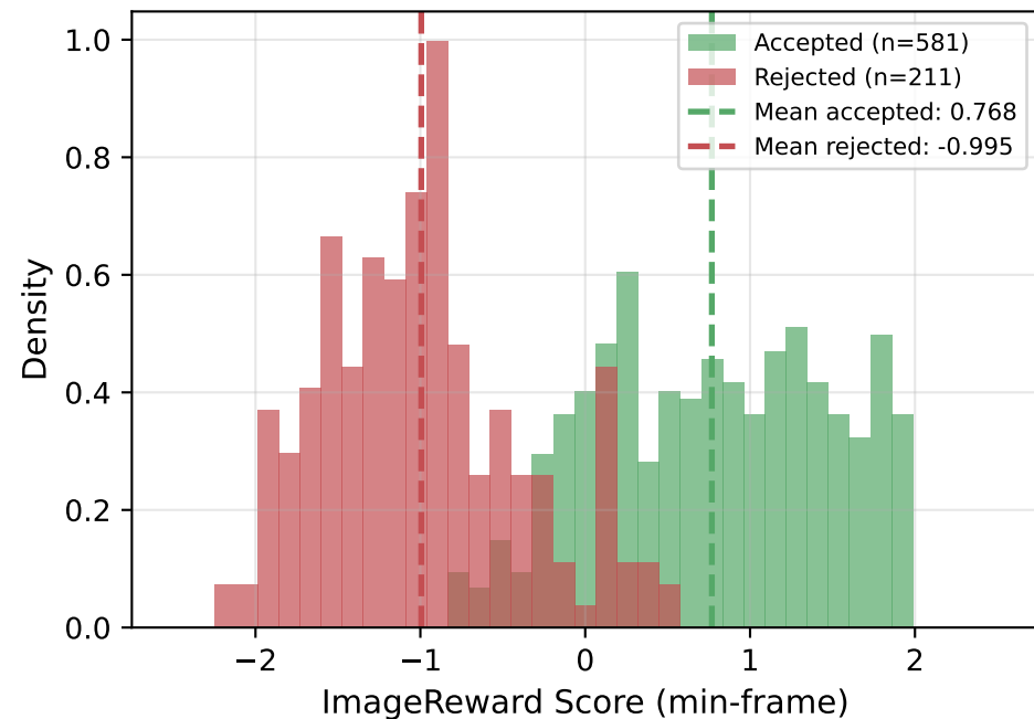
ImageReward Score Distribution for Accepted vs. Rejected Draft Blocks
