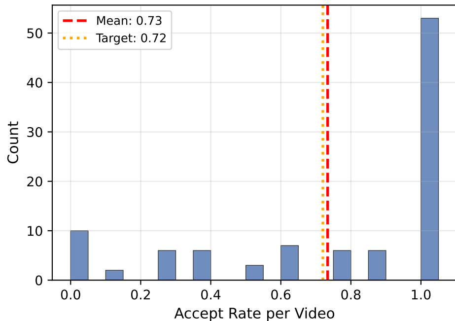
Per-Video Accept Rate Distribution (n=99 videos)
