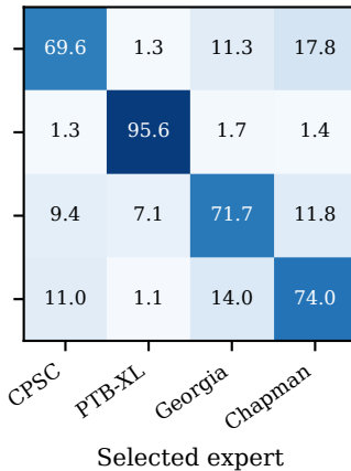
Shrinkage LDA
