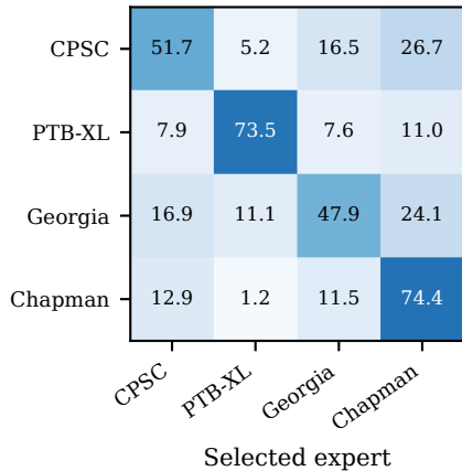
Centroid
