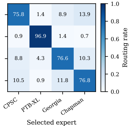
Domain MLP
