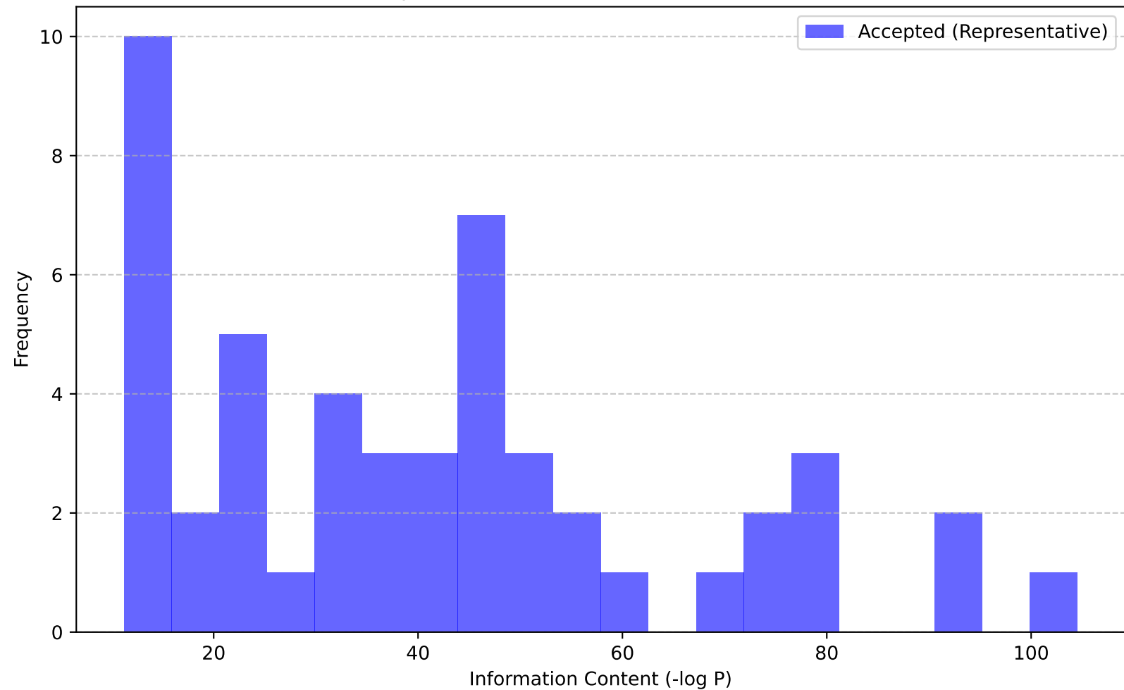
Representativeness of Model ( \tau=0.95 )
