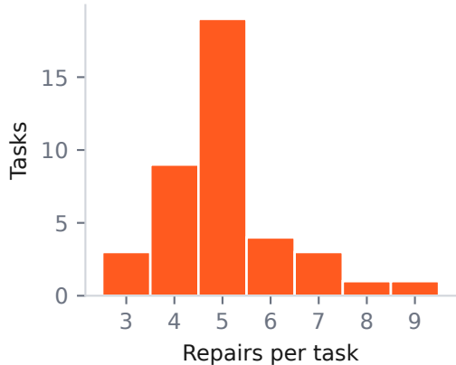
Task density
