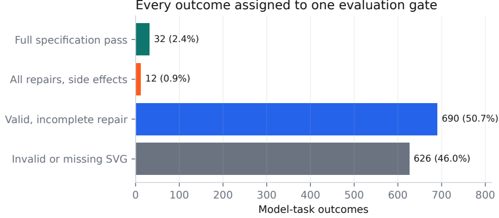
Figure 5: Mutually exclusive decomposition of all 1360 outcomes. The first two rows distinguish clean specification success from completed repairs with side effects; the remaining rows isolate incomplete valid edits from invalid or missing artifacts.
