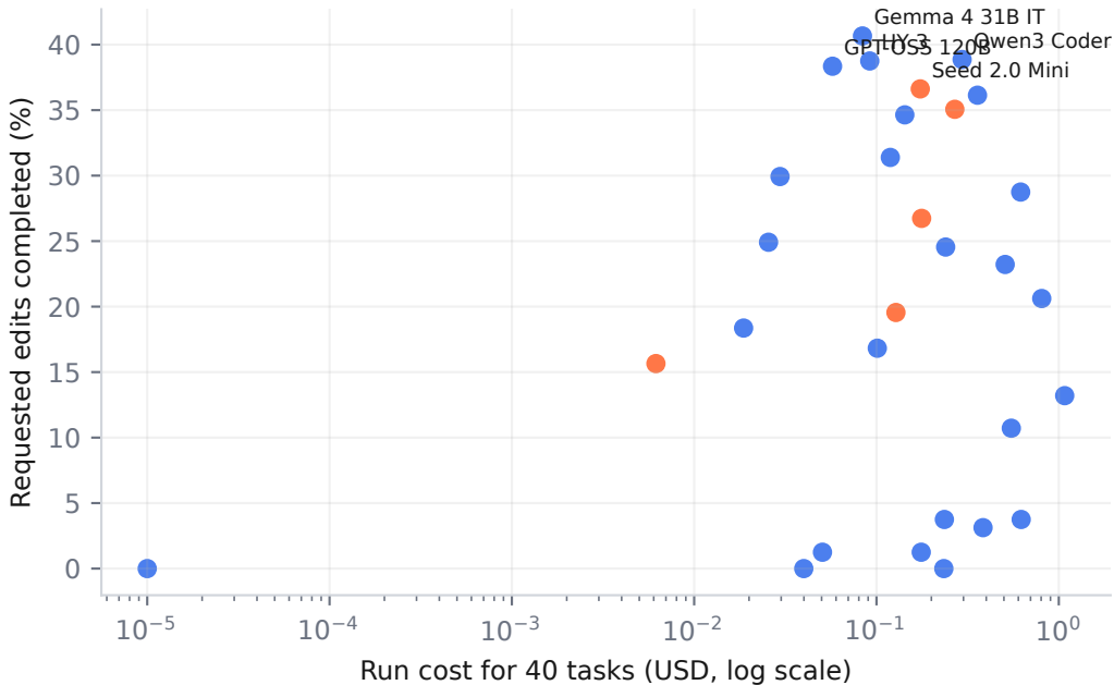
Quality-cost trade-off
