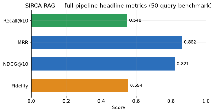
Fig. 2. Full-pipeline headline metrics on the 50-query benchmark.
