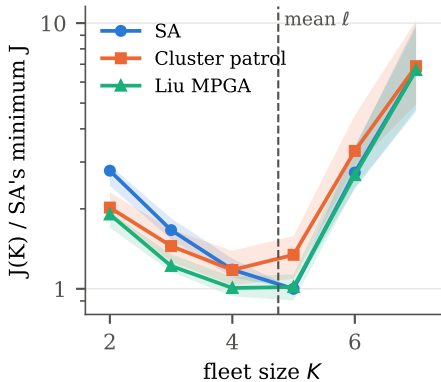
Clustered (paper)
