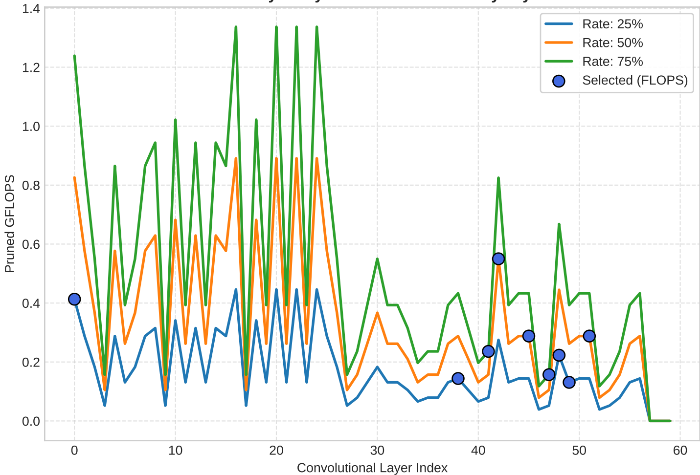
Sensitivity Analysis: Pruned GFLOPs by Layer
