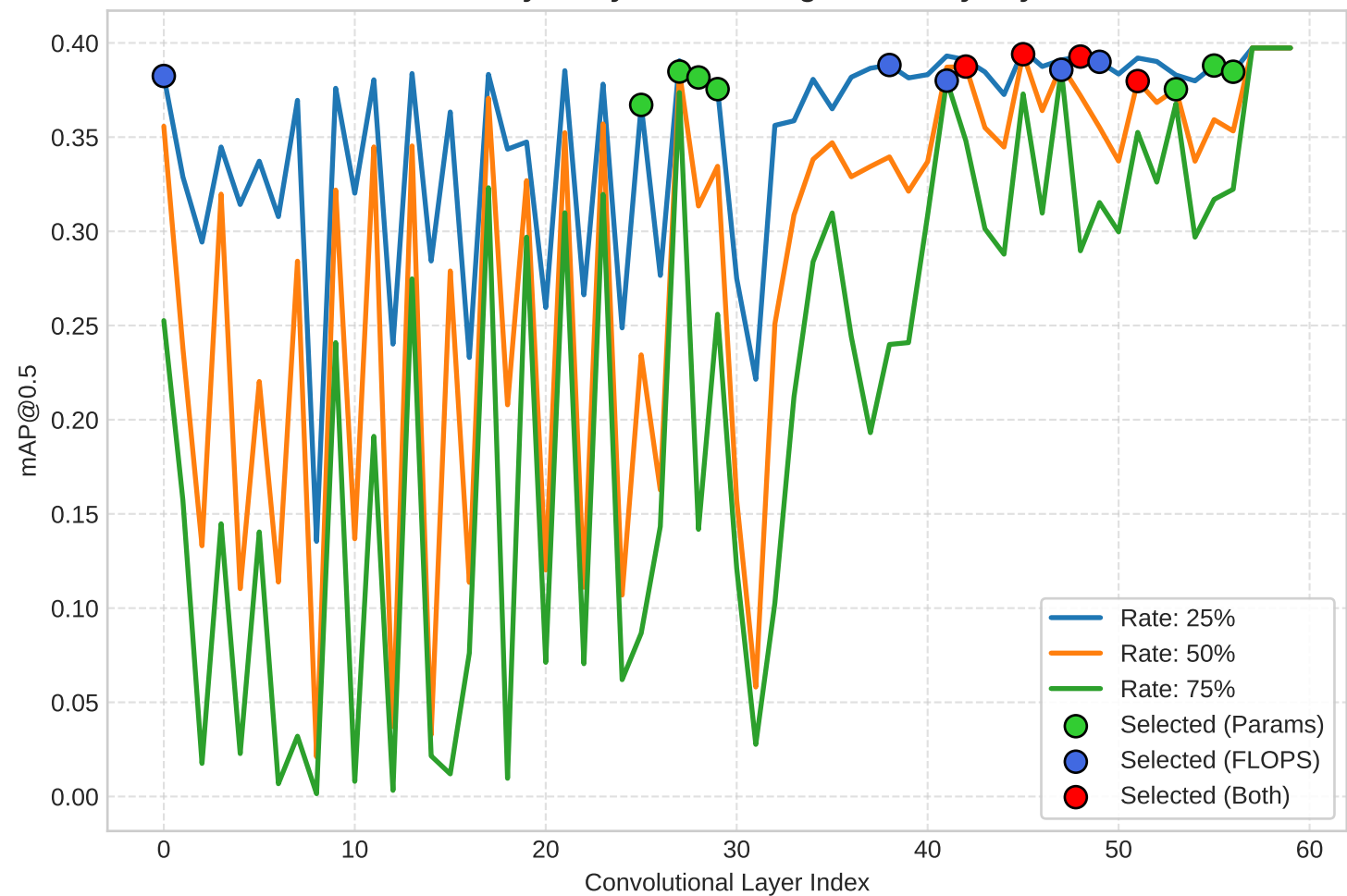
Sensitivity Analysis: mAP Degradation by Layer
