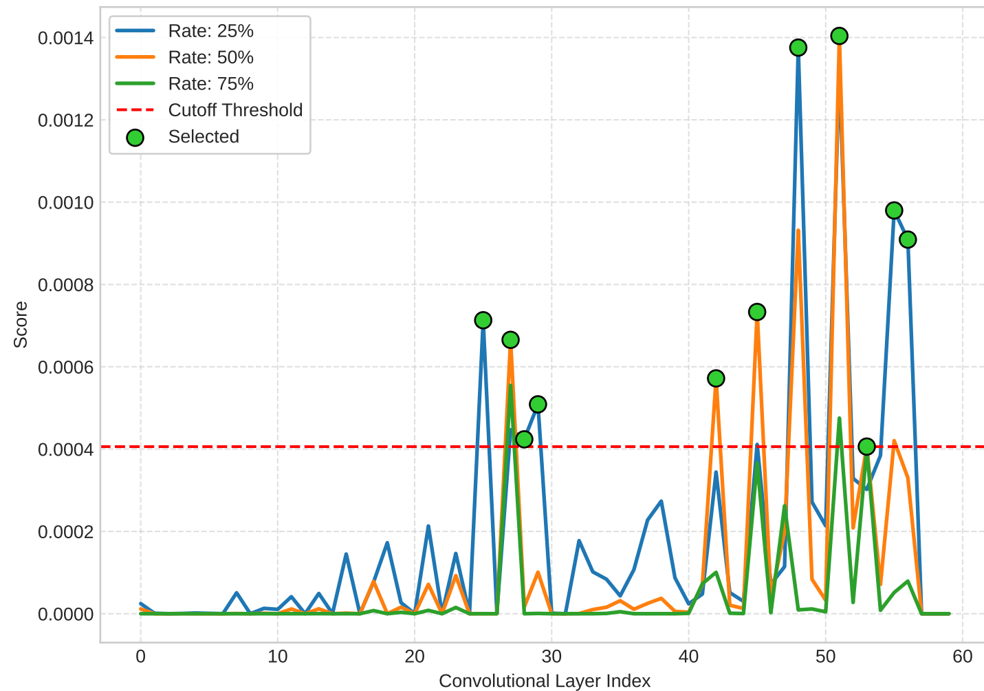
Parameter Selection Score: ParamsSaved * mAP^20
