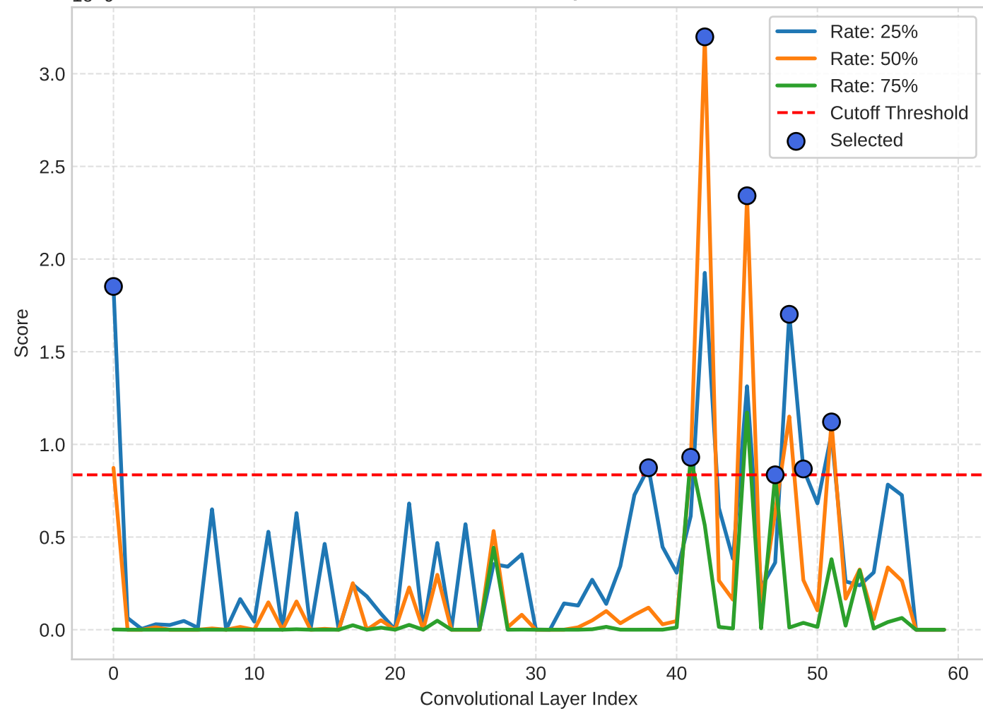
FLOPS Selection Score: FlopsSaved * mAP^20
