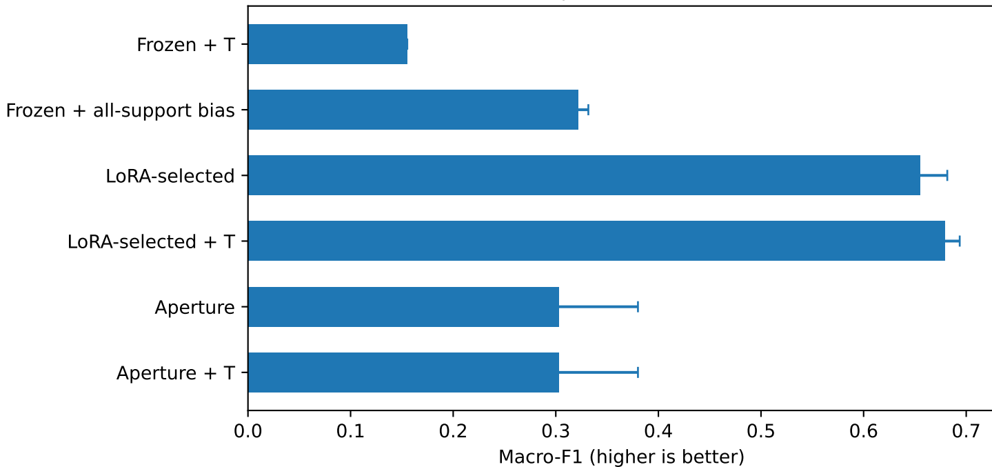
droid pick place | same total labeled budget
