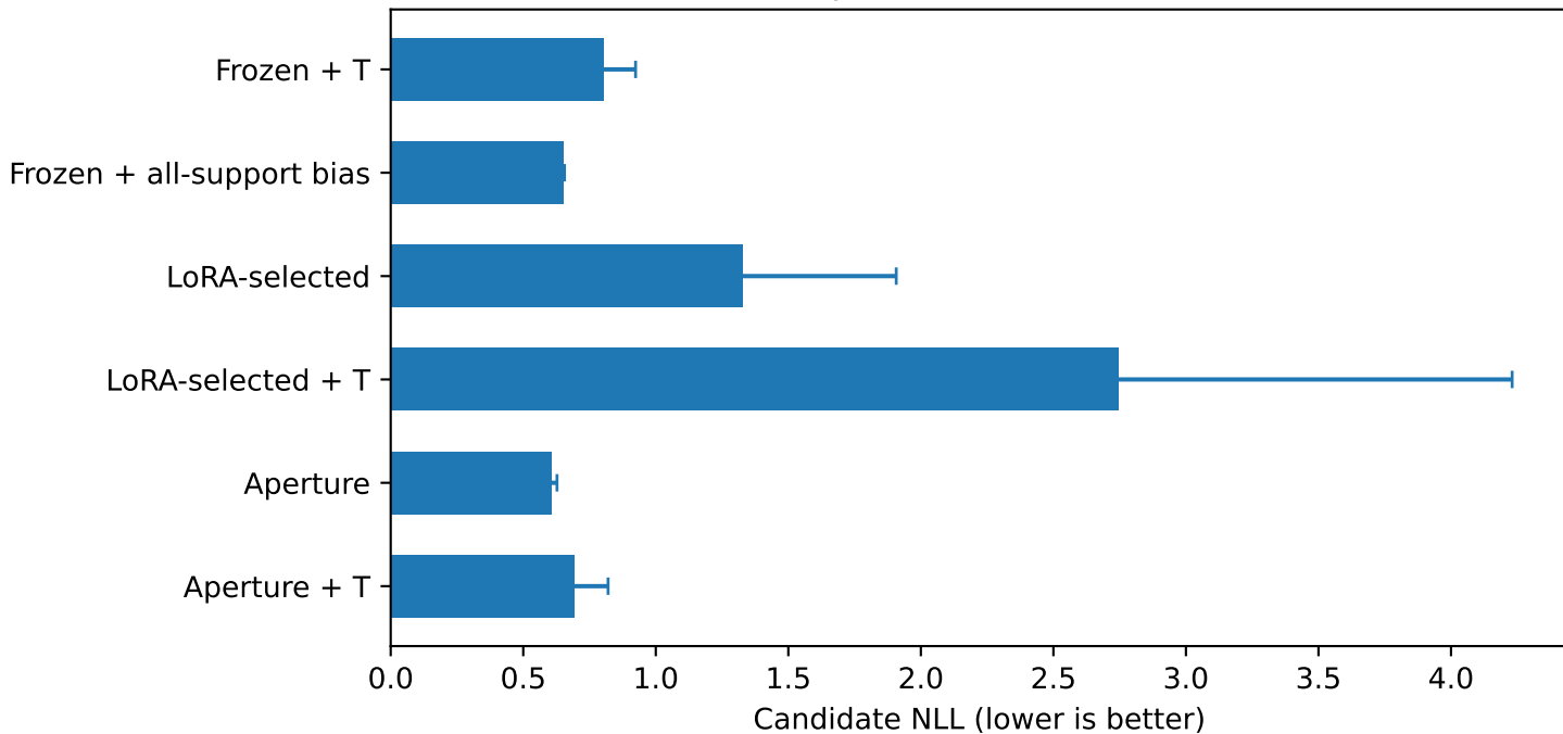
hospital 2 | same total labeled budget
