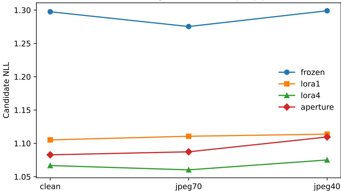
hawaii-wildfire | fixed-state 60-query probe
