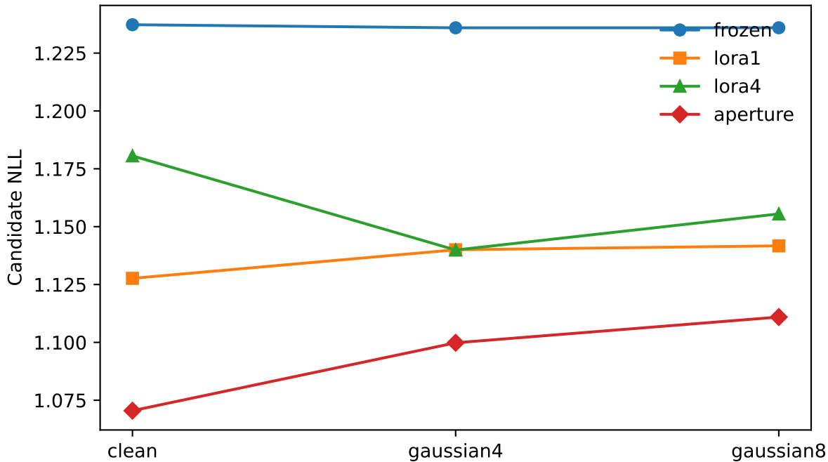
noto-earthquake | fixed-state 60-query probe
