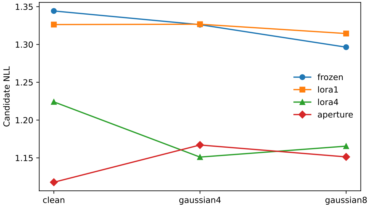
turkey-earthquake | fixed-state 60-query probe
