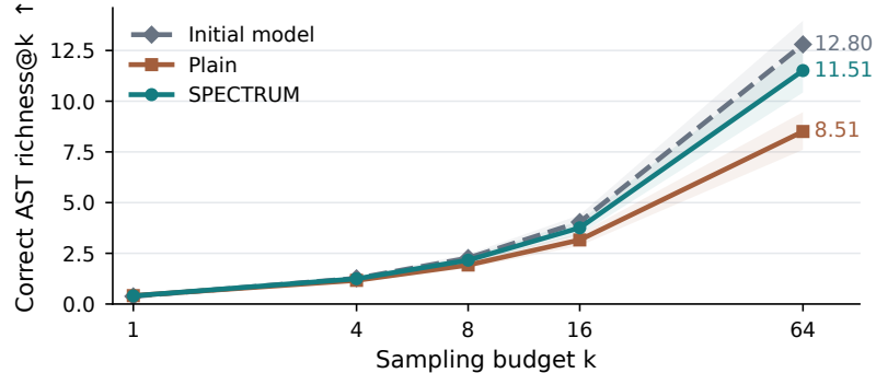
(a) More samples expose more retained implementations
