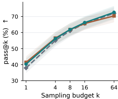
(b) Success probability
