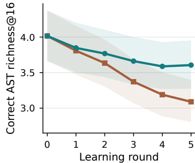
(b) All 500 tasks
