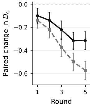
(b) Equal successes
