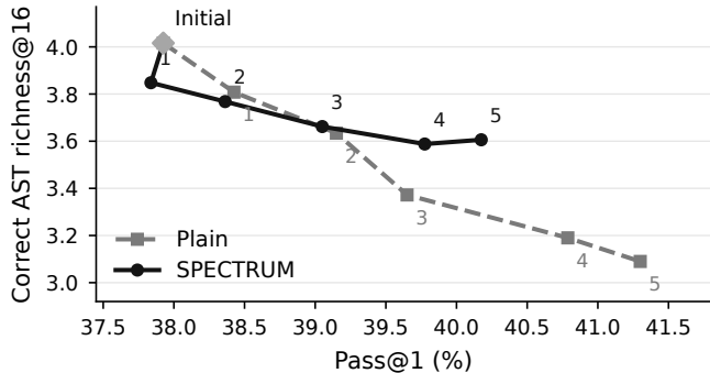
(a) More accurate, fewer correct structures
