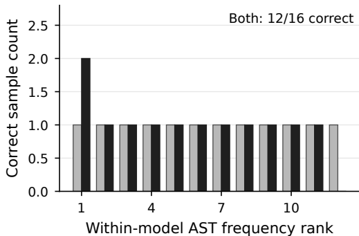
(b) HumanEval/2: a counterexample
