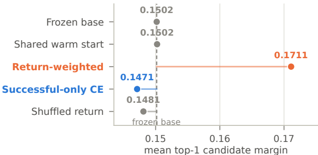
(a) what the objective optimises
