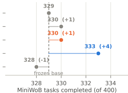
(b) what the agent actually does
