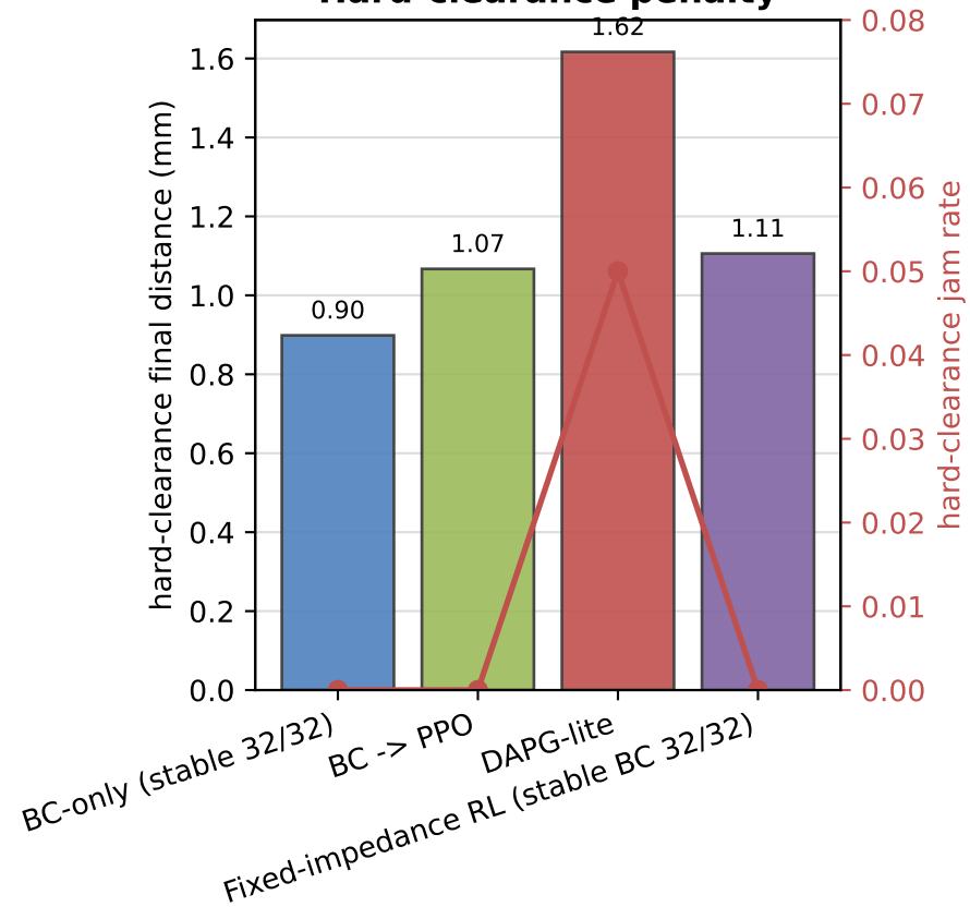
Hard-clearance penalty
