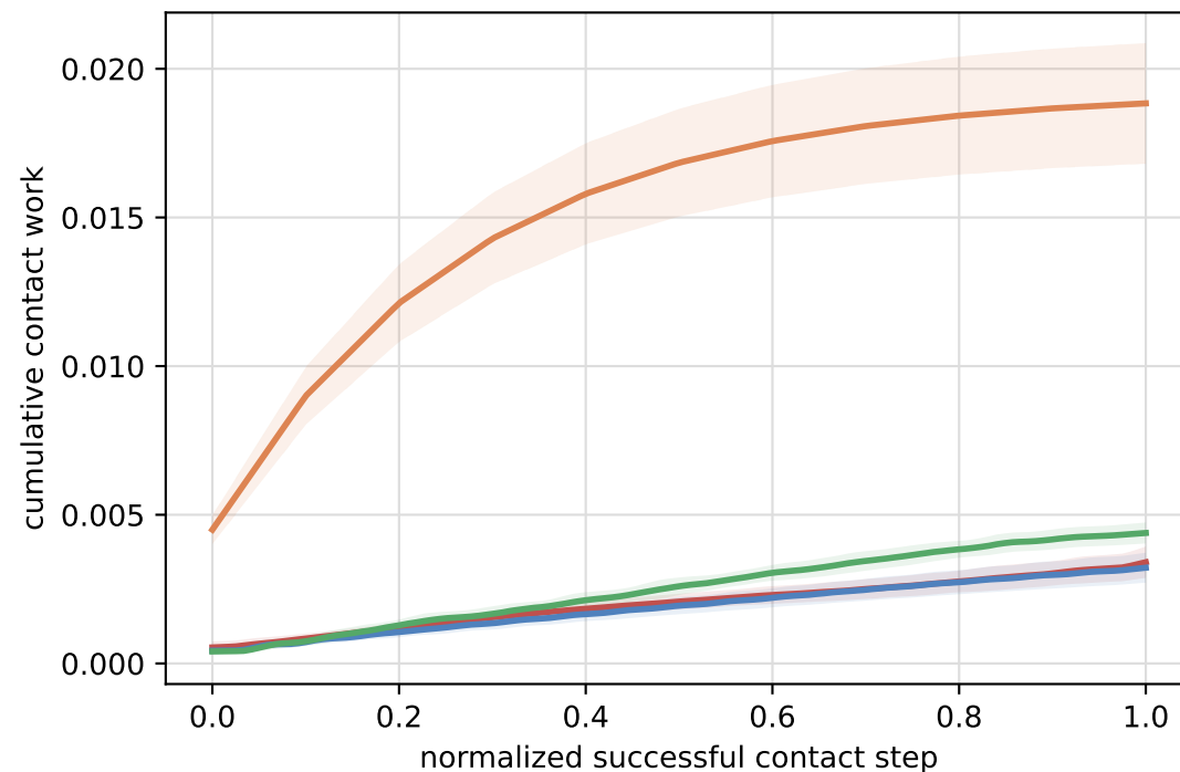
Success-matched work curve
